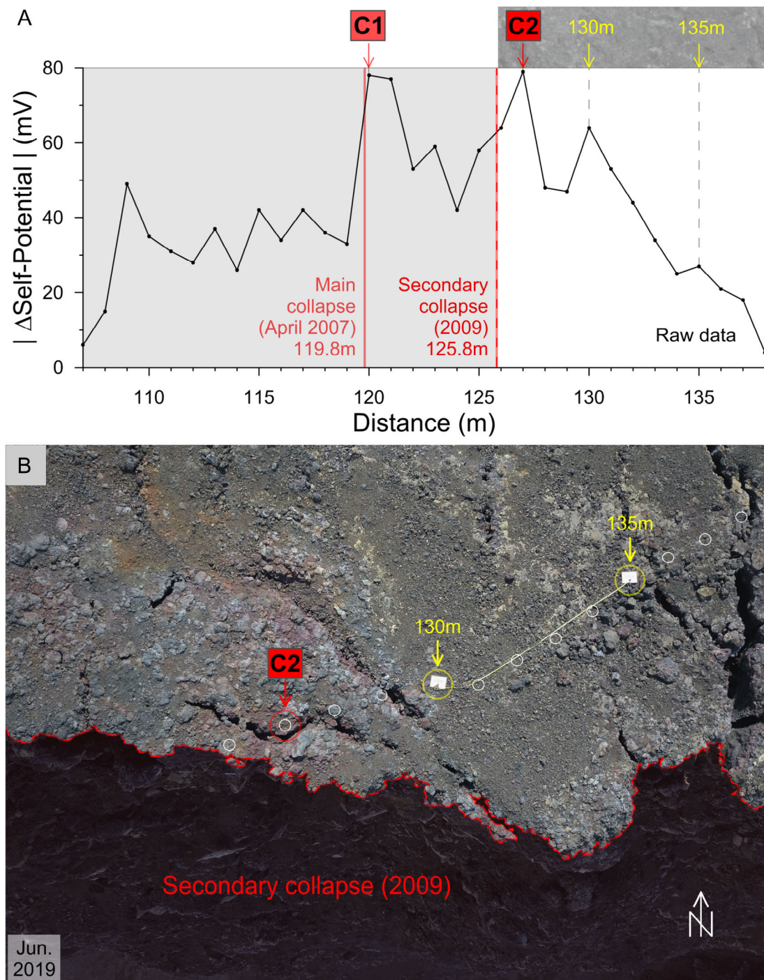
Figure 3: [A] Graph of the raw \Delta \text{SP} values centered on anomaly C, showing the two peaks, C1 and C2, both correlated at the meter scale with collapses of the Dolomieu caldera, in 2007 (main collapse) and in 2009 (secondary major rockfall). [B] Aerial photograph of the study area after the secondary rockfalls, showing the anomaly C2 at 1.2 m from the collapsed area (photo: R. Gusset).
