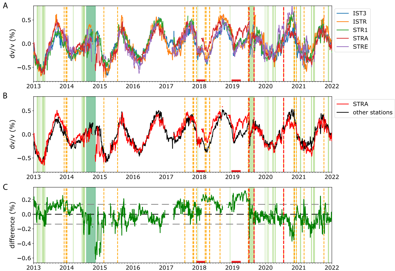
Figure 5: Comparing 2.0–4.0 Hz velocities (stretching technique) recorded at STRA station with other four stations. Volcanic activity described by red-dashed-lines = paroxysms, orange-dashed-lines = major explosions, light-green-shading = lava flows, dark-green shading = 2014 flank eruption. Red bars above date-axis indicate timing of raised alert level in late 2017 and late 2018. [A] Single-station seismic velocities for all stations. [B] Velocities for STRA station compared with average of IST3, ISTR, STR1, and STRE stations. [C] Difference between average velocity of STRA and other four stations. Grey dashed-lines represent one standard deviation of all calculated differences over the nine years either side of zero (black dashed-line).
