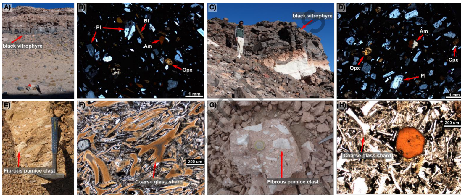
Figure 3: Characteristic macro- and microscopic features of the Río Frío (RF-2), Vega Helada (VH-2), Pajonales (PAJ-3), and Juncalito (Junc-2) ignimbrites. A) Field photograph of the Río Frío ignimbrite (RF-2), showing welded crystal lapilli-tuff layers, including a black vitrophyre. B) Thin section of RF-2 with plagioclase, orthopyroxene, amphibole, and scarce biotite in a glassy matrix. C) Field photograph of the Vega Helada ignimbrite (VH-2), likewise displaying variations in welding grade, including in a vitrophyre. D) Thin section of VH-2 with plagioclase, clinopyroxene, orthopyroxene, and scarce amphibole in a glassy matrix. E) Hand specimen of the Pajonales ignimbrite (PAJ-3) with characteristically abundant fibrous pumice fragments. F) Thin section of PAJ-3 showing scarce phenocrysts in a coarse, glass shard-rich matrix. G) Hand specimen of the Juncalito ignimbrite (Junc-2) with abundant fibrous pumice fragments. H) Thin section of Junc-2 with sparse phenocrysts in a coarse, glass shard-rich matrix. Mineral abbreviations follow Siivola and Schmid (2007): Pl = plagioclase, Am = amphibole, Bt = biotite, Opx = orthopyroxene, Cpx = clinopyroxene.
