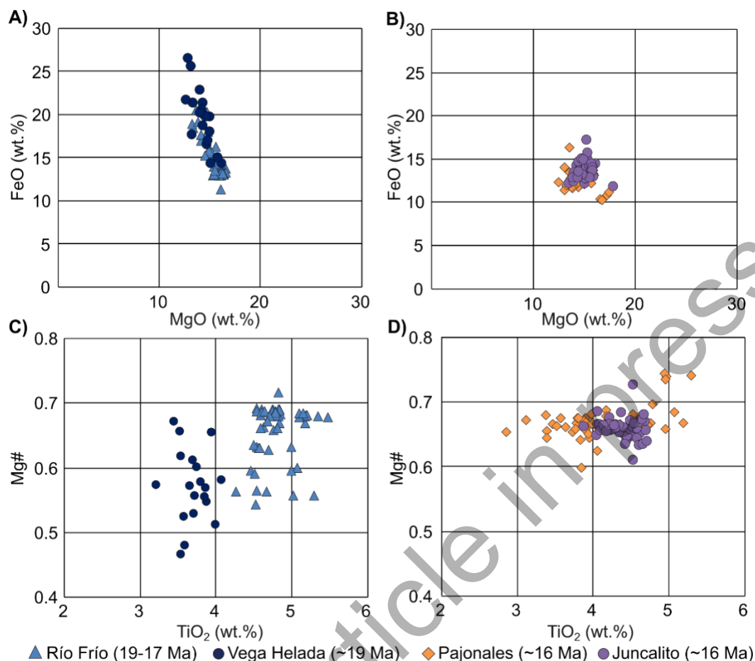
Figure 8: Specific biotite chemistry comparison diagrams for the main proximal correlation issues discussed in this study. A) FeO vs MgO diagram comparing the Río Frío (RF) and Vega Helada (VH) ignimbrites. B) FeO vs MgO diagram comparing the Pajonales (PAJ) and Juncalito (Junc) ignimbrites. C) Mg# vs TiO 2 diagram for Río Frío and Vega Helada. D) Mg# vs TiO 2 diagram for Pajonales and Juncalito. Mg# is defined as Mg/(Mg + Fe_{total}) , calculated on a molar basis from structural-formula cations, where Fe total represents total iron. Oxide concentrations are expressed in wt.%.
